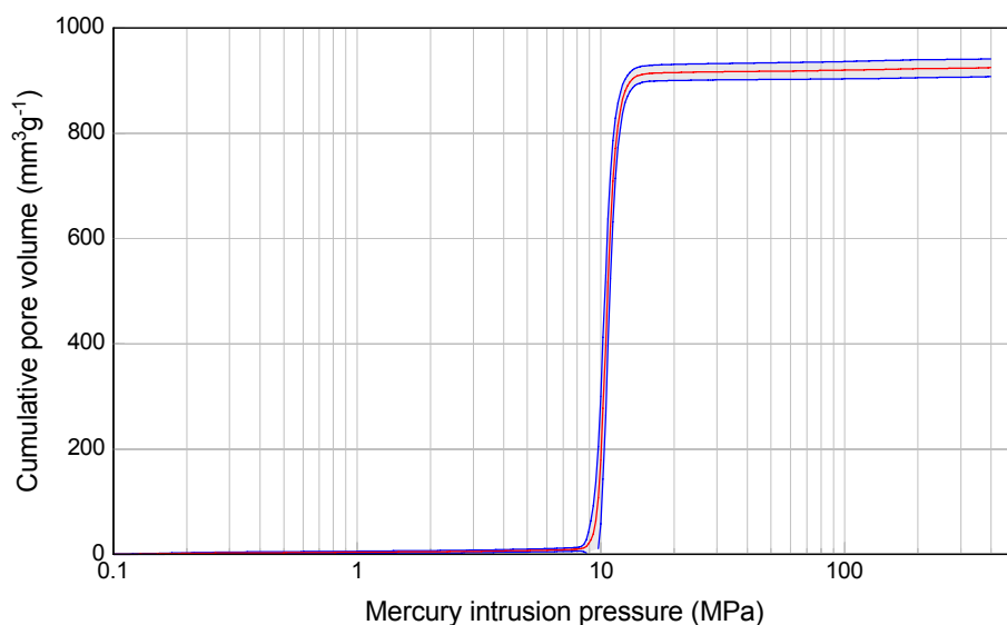
Figure A1: Certified pressure-volume curve of material ERM ® -FD122 with uncertainty interval
