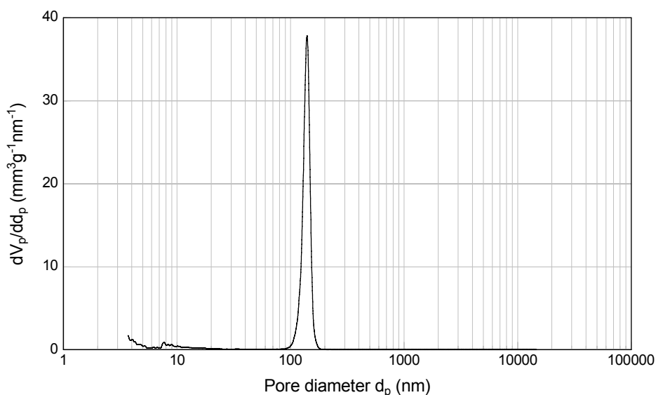
Figure 1: Pore size distribution of ERM ® -FD122 (non-certified)
